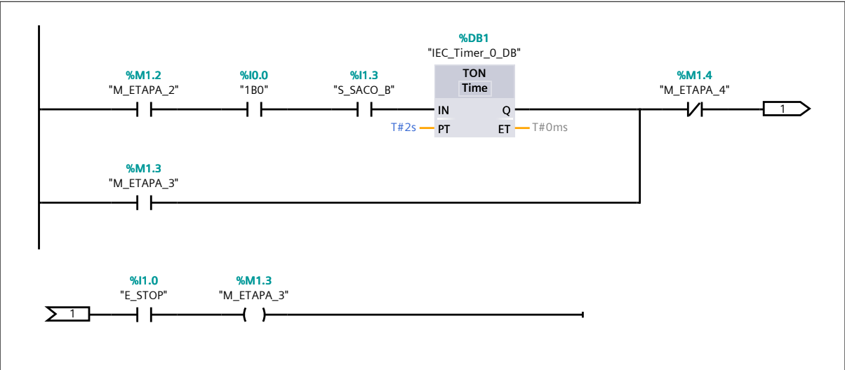
Network 8: Avance Cilindro 2
